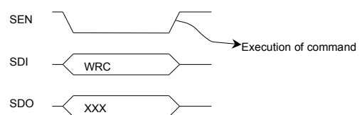
Figure 11: SPI command execution
