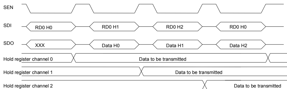
Figure 9: SPI read access 16Bit
