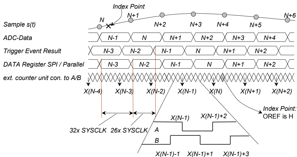
Figure 14: propagation delay
