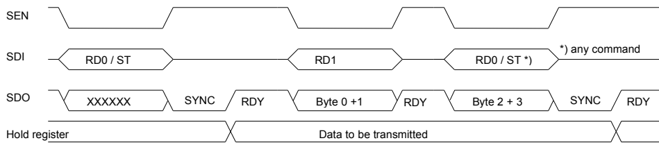
Figure 8: SPI read access 32Bit
