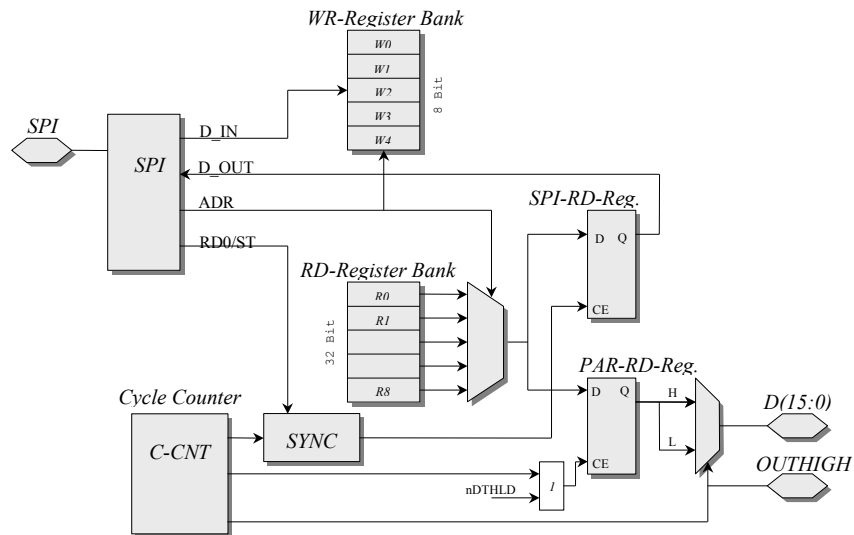
Figure 6: interface structure
