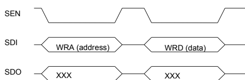
Figure 10: SPI write access
