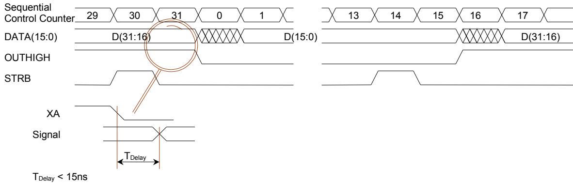
Figure 12: timing Parallel Data Port
