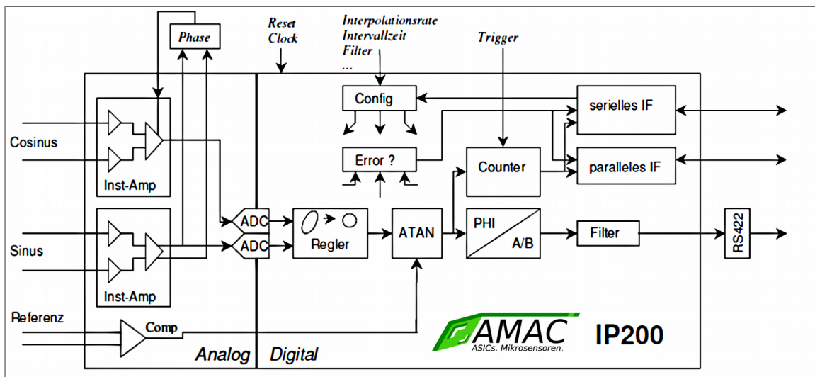
Figure 1: block diagram
