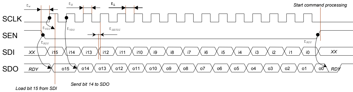
Figure 7: SPI timing
