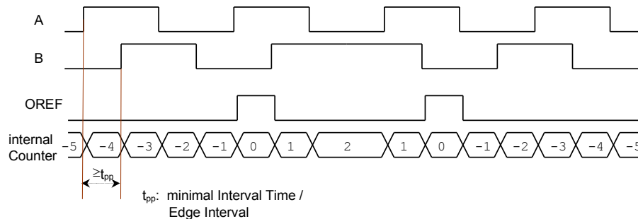
Figure 5: Output Signals / Counter Value
