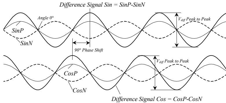
Figure 2: Input Signals
